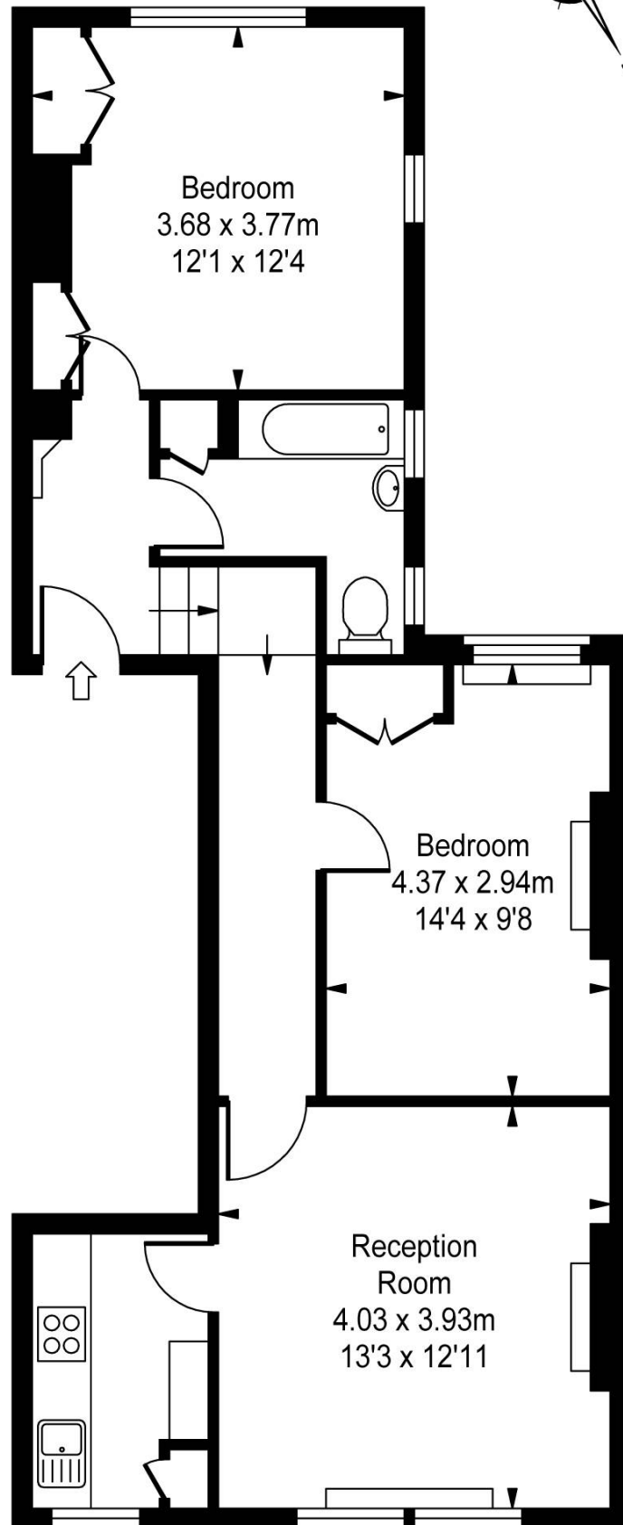
First Floor
